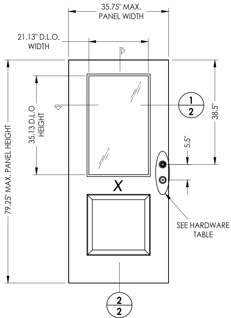
40 FIBERGLASS DOOR PANEL GlassCraft
