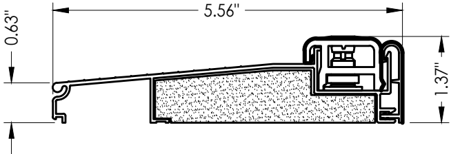
14 INSWING THRESHOLD WORLDWIDE 99-558
